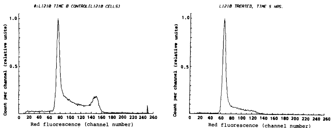
Figure 3. Flow cytometric DNA analysis of L1210 cells treated with 10 \mu M vibriobactin.
