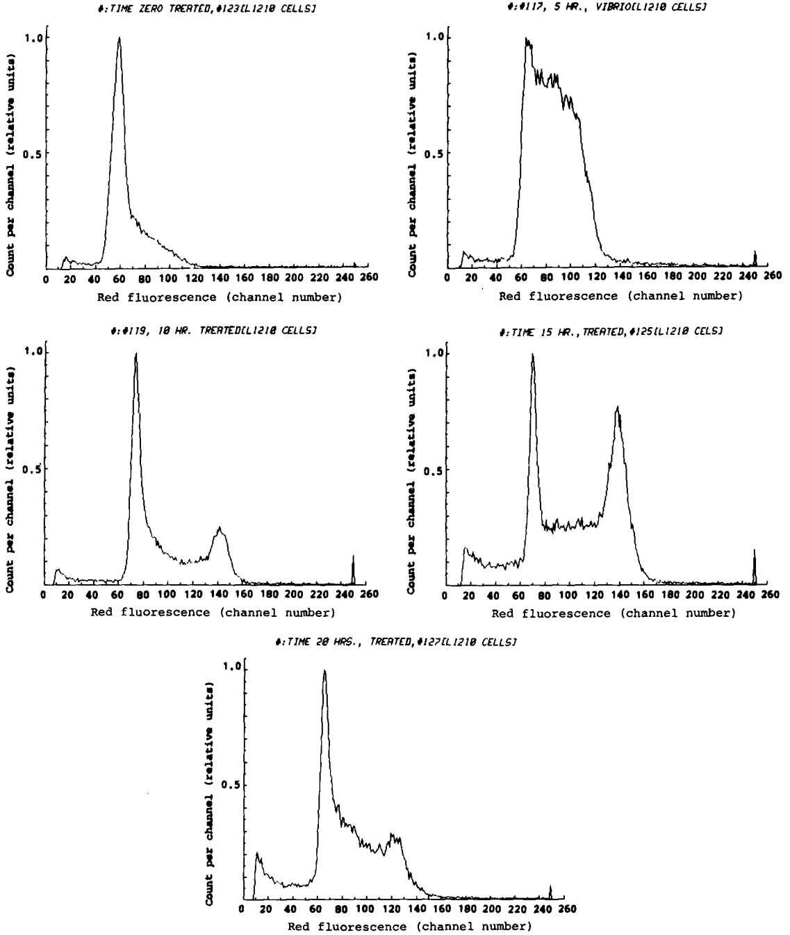
Figure 4. Flow cytometric DNA analysis of L1210 cells regrown in fresh media after treatment with 10 \mu M vibriobactin for 5 hrs.
